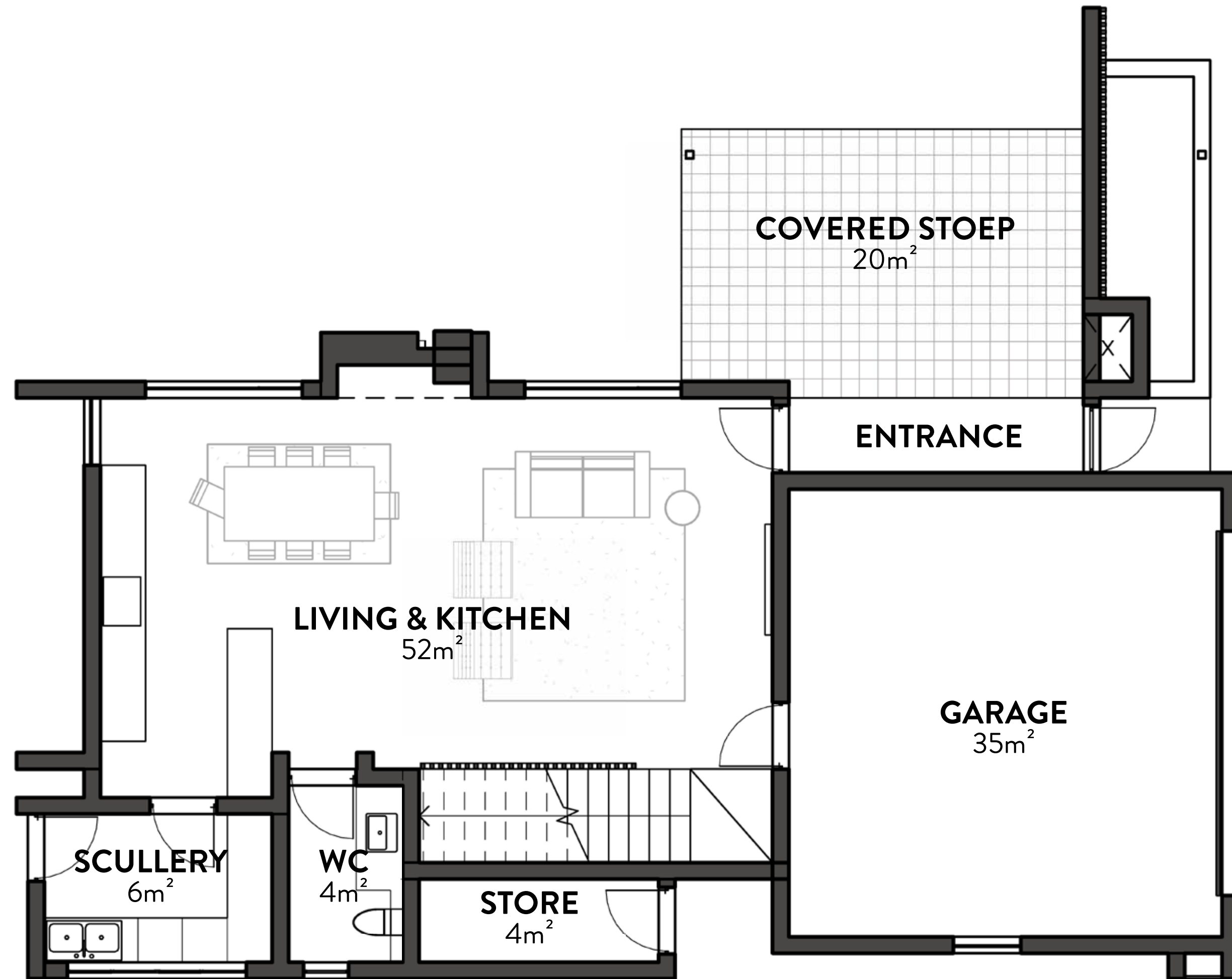
GROUND FLOOR
